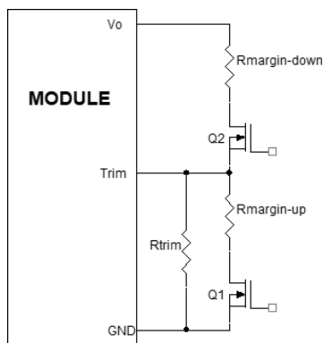
Figure 41. Circuit Configuration for margining Output voltage
