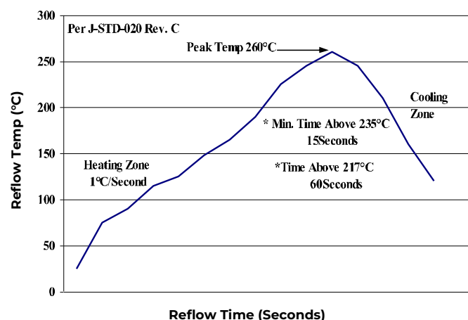
Figure 19. Recommended linear reflow profile using Sn/Ag/Cu solder.
