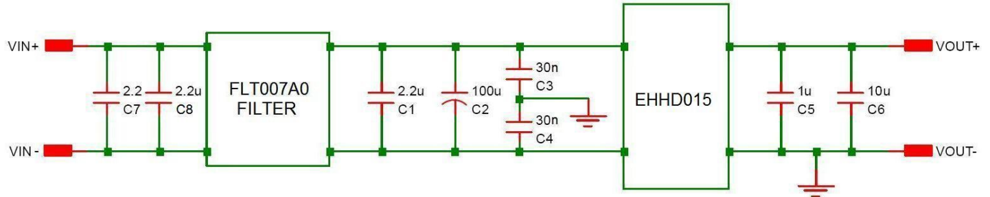
Figure 20. EMC Considerations
