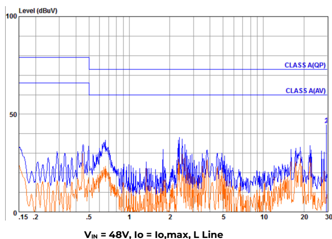
Figure 22. EMC Considerations
