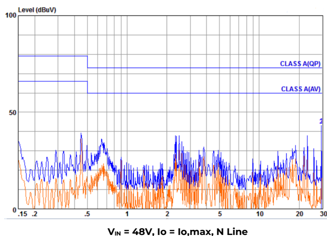
Figure 22. EMC Considerations
