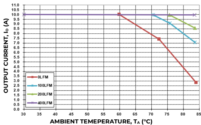
Figure 16a. Output Current Derating for the Module with Heatplate; Airflow in the Transverse Direction from V_{out}(+) to V_{out}(-) ; V_{IN}=48V .
