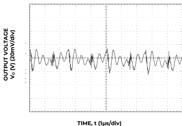
Figure 2. Typical output ripple and noise ( C_o=10\mu\text{F} ceramic, V_{IN}=8\text{V} , I_o=I_{o, \text{max}} ).
