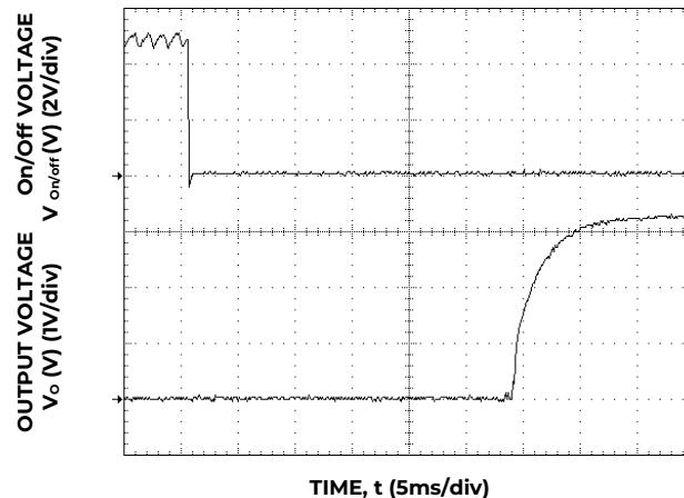
Figure 11. Typical Start-up Using Remote On/Off, negative logic version shown ( V_{IN} = V_{IN,NOM} , I_o = I_{o,max} ).
