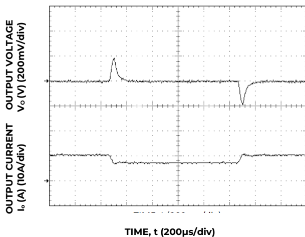
Figure 3. Transient Response to Dynamic Load Change, 0.1A/μs, from 75% to 50% to 75% of full load.
