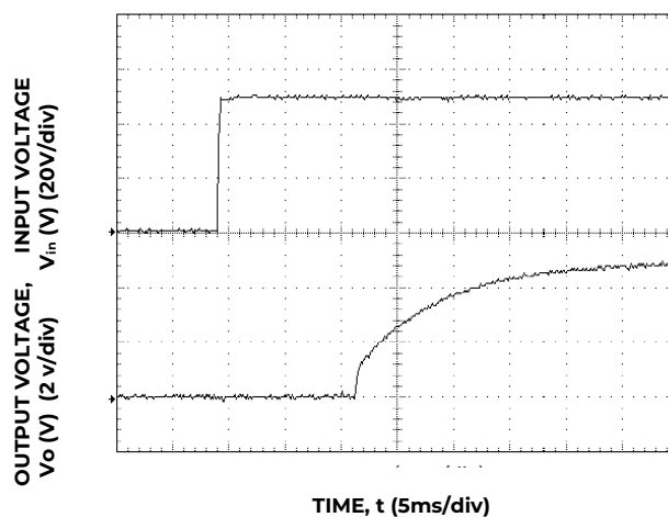
Figure 6. Typical Start-up Using Input Voltage ( V_{IN}=V_{IN, \text{NOM}} , I_o=I_{o, \text{max}} ).
