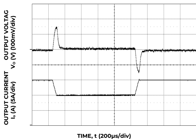
Figure 9. Transient Response to Dynamic Load Change, 0.1A/μs, from 75% to 50% to 75% of full load.
