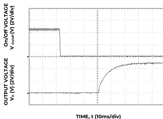
Figure 5. Typical Start-up Using Remote On/Off, negative logic version shown ( V_{IN}=V_{IN, \text{NOM}} , I_o=I_{o, \text{max}} ).
