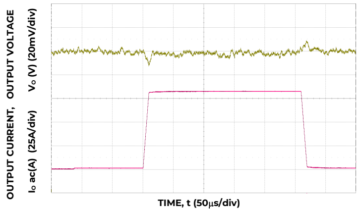
Figure 22. Trans. Resp. to 100A/μs Load Change from 25% to 75% at 12V IN , C o =4x0.047μF +4x0.1μF + 15x22μF + 73x47μF + 6x470μF polymer.
