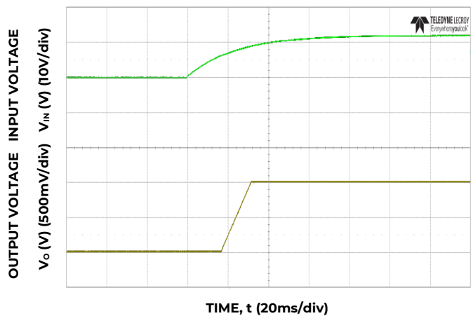
Figure 12. Typical Start-up Using Input Voltage ( V_{IN}=12\text{V} , I_o=I_{o,max} ).
