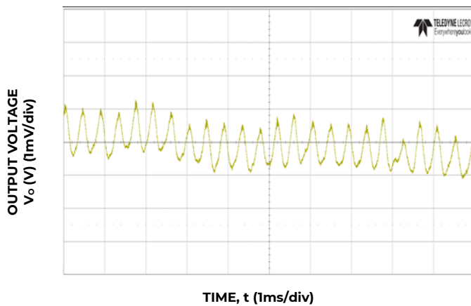
Figure 9. Typical output ripple( C_o=4\times0.047\mu\text{F}+4\times0.1\mu\text{F}+15\times22\mu\text{F}+73\times47\mu\text{F}+6\times470\mu\text{F} polymer, V_{IN}=12\text{V} , I_o=I_{o,max} ).
