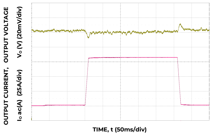
Figure 10. Trans. Resp. to 100A/μs Load Change from 25% to 75% at 12V IN , C_o=4\times0.047\mu\text{F}+4\times0.1\mu\text{F}+15\times22\mu\text{F}+73\times47\mu\text{F}+6\times470\mu\text{F} polymer.
