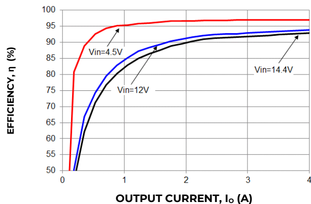
Figure 25. Converter Efficiency verses output current
