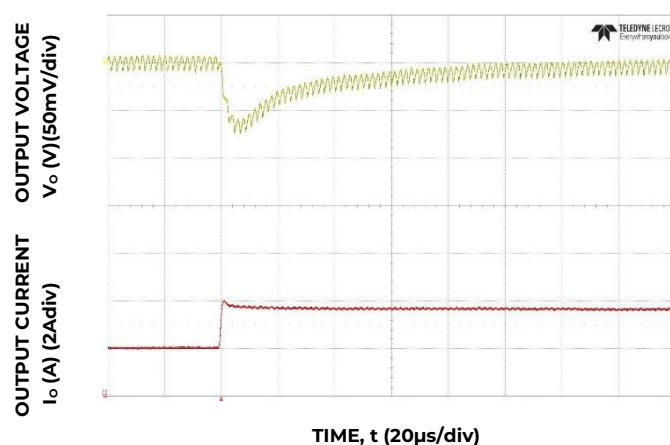
Figure 28 Transient Response to Dynamic Load Change from 50% to 100% at 12Vin, C_{out}=3 \times 47\mu F , C_{Tune}=470pF , R_{Tune}=300
