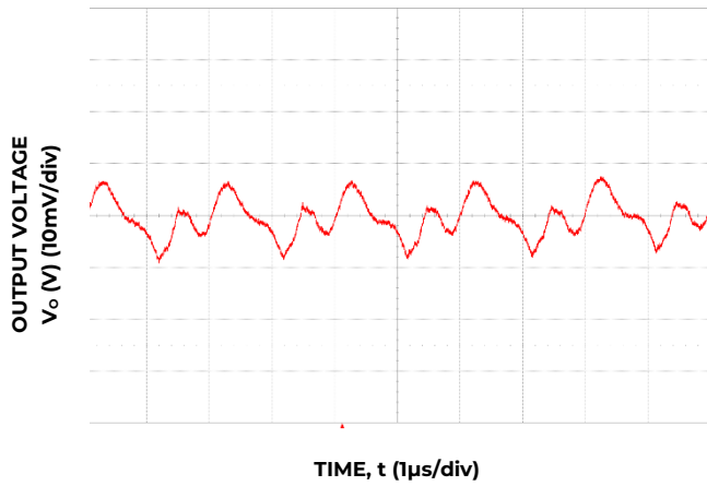
Figure 15. Typical output ripple ( C_o=3 \times 22\mu F ceramic, V_{IN} = 12V , I_o = I_{o,max} ).
