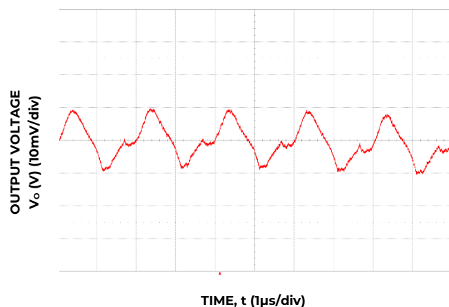
Figure 27. Typical output ripple and noise ( C_o=3 \times 22\mu F ceramic, V_{IN}=12V , I_o = I_{o,max} ).
