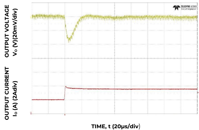
Figure 16. Transient Response to Dynamic Load Change from 50% to 100% at 12Vin, C_{out}=5 \times 47\mu F , C_{Tune}=4.7nF , R_{Tune}=300
