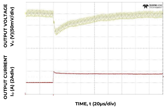
Figure 34. Transient Response to Dynamic Load Change from 50% to 100% at 12Vin, C_{out}=2 \times 47\mu\text{F} , C_{Tune}=220\text{pF} , R_{Tune}=300
