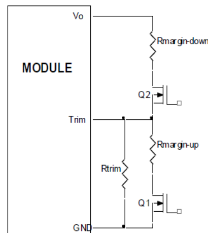
Figure 43. Circuit Configuration for margining Output voltage.
