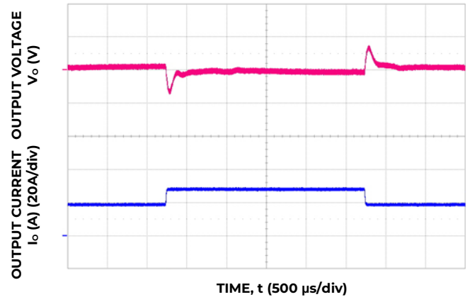
Figure 4. Typical Transient Response to 1A/μs Step Change in Load from 50% to 75% to 50% of Full Load, C_o = 1440\mu F and 50 V dc Input
