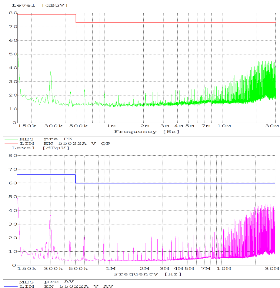
Figure 22. EMC Considerations
