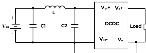
Figure 11. EMI with filter
