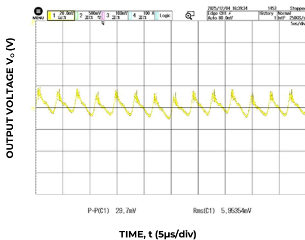
Figure 3. Typical output ripple and noise ( C_o = 350\mu F Ceramic + 2200μF PosCap Oscon, V_{in} = 54V , I_o = I_{o,max} )
