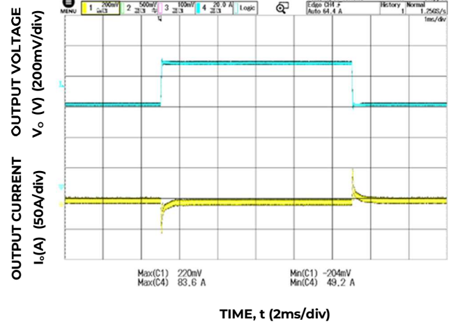
Figure 4. Dynamic Load Response, dI_o/dt=1A/\mu s ; V_{in}=54V ; T_A=25^\circ C ; Load I_o = 50\% to 75\% of I_{o,max} ; C_o = 350\mu F Ceramic +4850μF Ploy CAP
