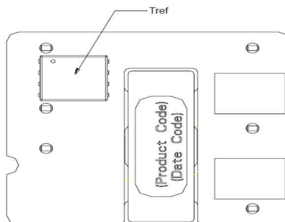
Figure 17. T_{ref} Temperature Measurement Location.
